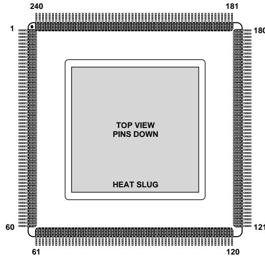
THE 240-LEAD PACKAGE CONTAINS A COPPER/TUNGSTON HEAT SLUG ON ITS TOP SURFACE.
