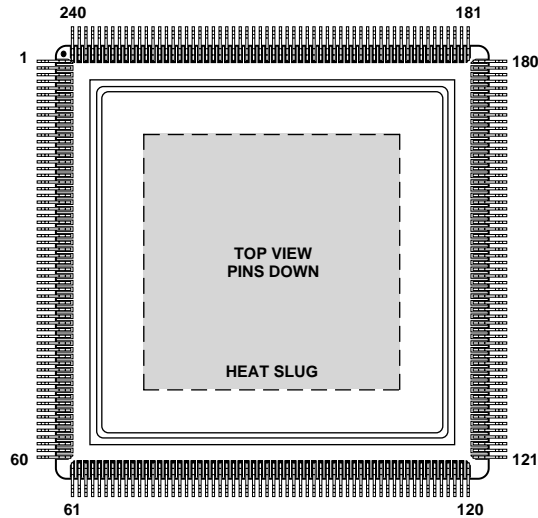
THE 240-LEAD PACKAGE CONTAINS A COPPER/TUNGSTON HEAT SLUG ON ITS BOTTOM SURFACE.
